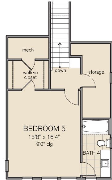
WESTWIND - Bedroom 5, Bath 4 i/l/o Bonus Room, Powder Bath - TOTAL LIVING: 4,064 S.F.
