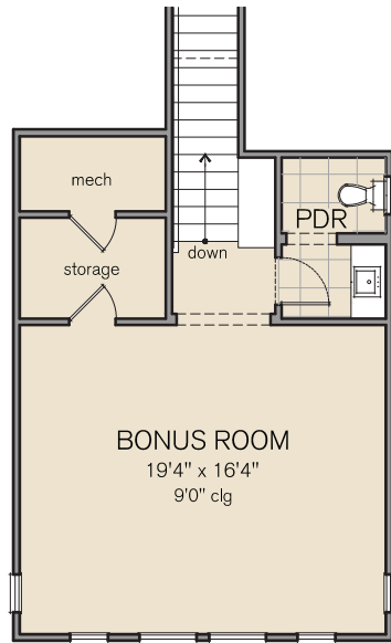
WESTWIND - Traditional Standard Second Floor Bonus Room, Powder Bath
