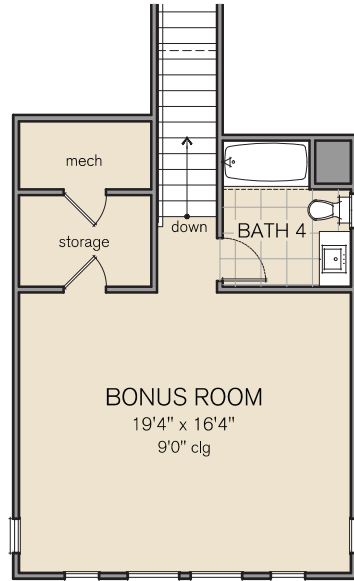
WESTWIND - Bath 4 i/l/o Powder Bath TOTAL LIVING: 4,064 S.F.
